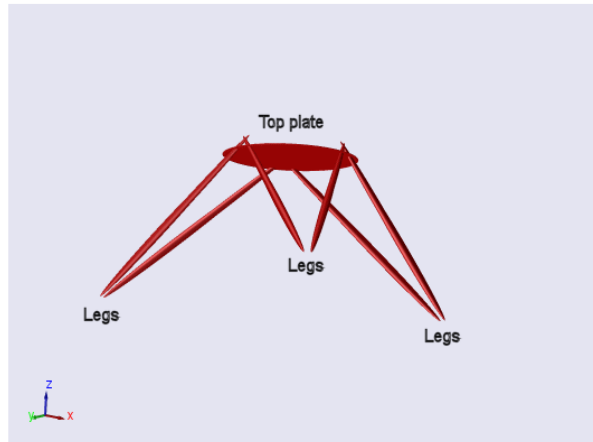
Stewart Platform: Bodies Displayed as Convex Hulls and as Equivalent Ellipsoids
